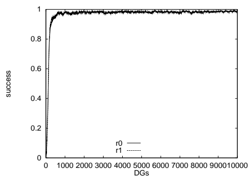
(a) Discriminative success
